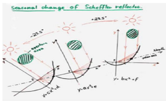
Different parabolas focus the sunlight at different seasons. The incident light has to be parallel to their y-axis. Note the seasonal change in the aperture area, focus "F" and the center of the Scheffler reflector (black dot) remain stationary
