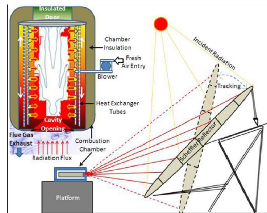
Fig 1: Block Diagram of Solar Crematorium
